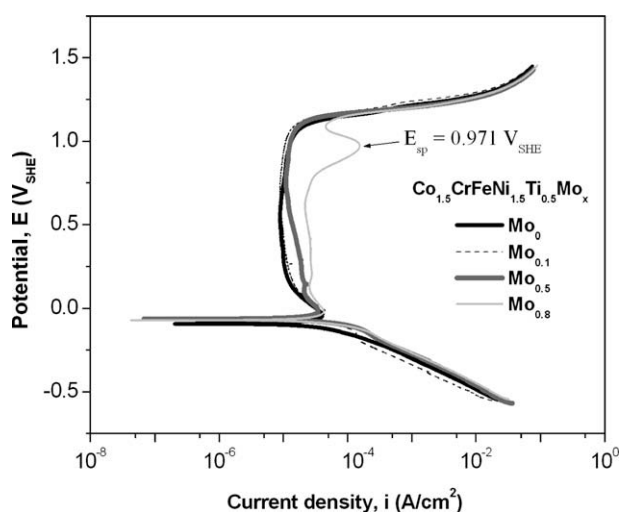
Fig. 3. Potentiodynamic polarisation curves of the \text{Co}_{1.5}\text{CrFeNi}_{1.5}\text{Ti}_{0.5}\text{Mo}_x alloys with various Mo contents ( x = 0, x = 0.1, x = 0.5 , and x = 0.8 mol) in deaerated 0.5 M \text{H}_2\text{SO}_4 .
