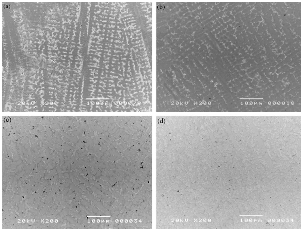
Fig. 2. SEM images of the as-cast \text{Co}_{1.5}\text{CrFeNi}_{1.5}\text{Ti}_{0.5}\text{Mo}_x high-entropy alloys: (a) x = 0 , (b) x = 0.1 , (c) x = 0.5 , and (d) x = 0.8 mol.
