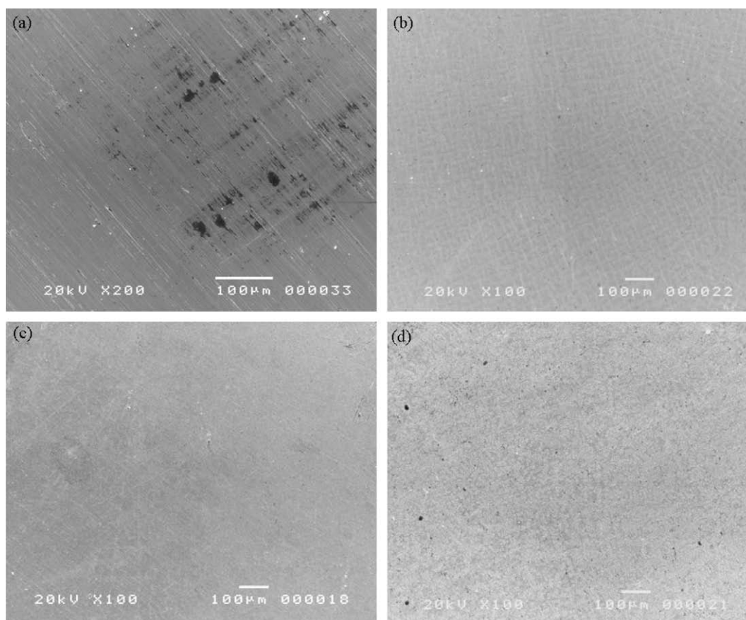
Fig. 7. SEM images of the \text{Co}_{1.5}\text{CrFeNi}_{1.5}\text{Ti}_{0.5}\text{Mo}_x high-entropy alloys: (a) x = 0 , (b) x = 0.1 , (c) x = 0.5 , and (d) x = 0.8 mol after potentiodynamic polarisation in deaerated 1 M NaCl.
