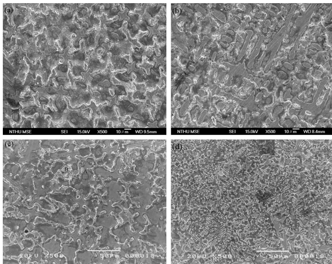
Fig. 6. SEM images of the \text{Co}_{1.5}\text{CrFeNi}_{1.5}\text{Ti}_{0.5}\text{Mo}_x high-entropy alloys: (a) x = 0 , (b) x = 0.1 , (c) x = 0.5 , and (d) x = 0.8 mol after potentiodynamic polarisation in deaerated 0.5 M \text{H}_2\text{SO}_4 .
